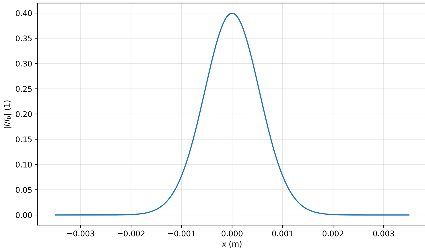
Intensity profile I(x, y = 0, z = 2.627m)/I_0 , P_{in}=0.1P_{cr} , artificial time
